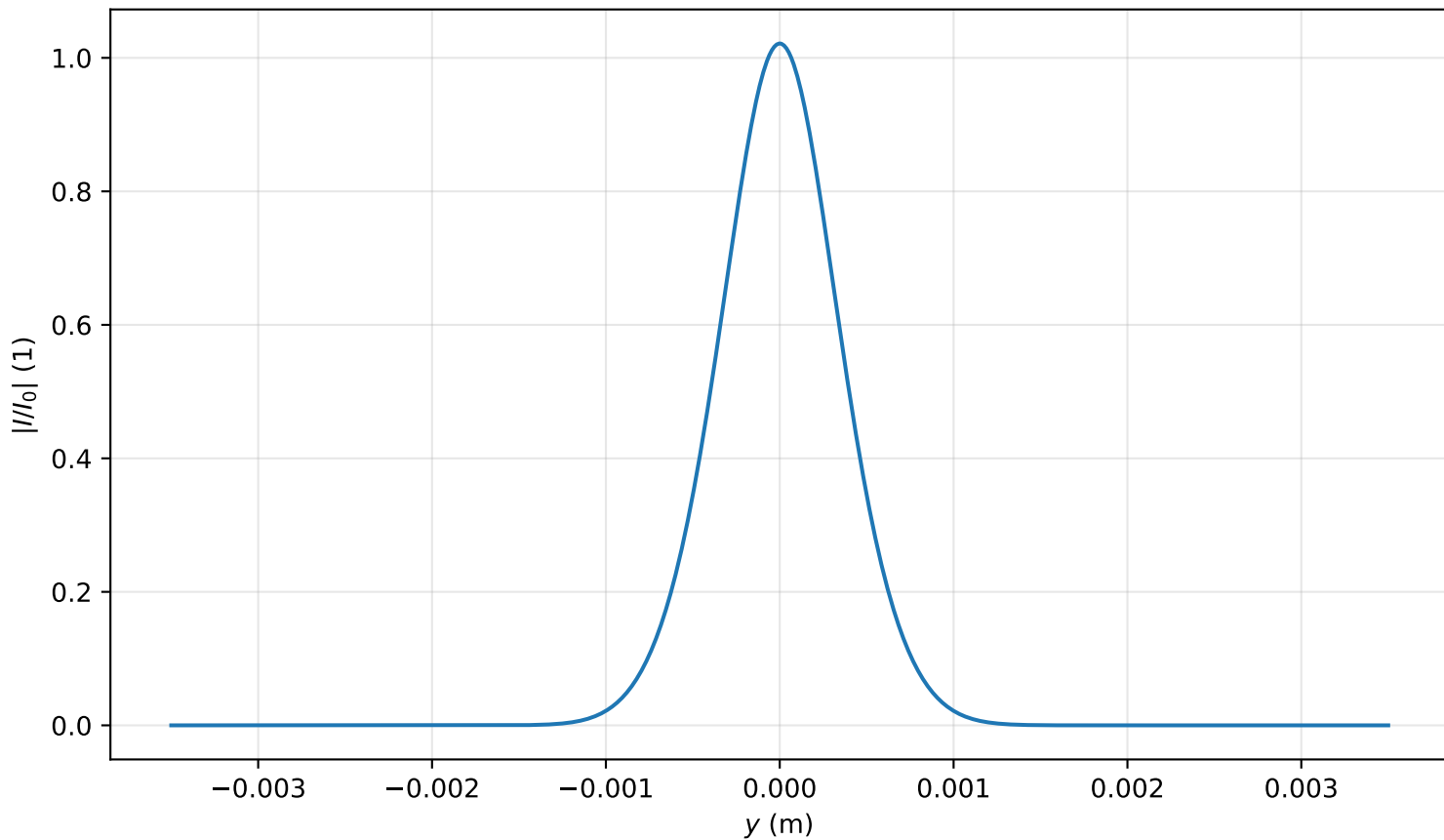
Intensity profile I(x=0, y, z=0.637)/I_0 , P_{in}=0.4P_{cr} , artificial time
